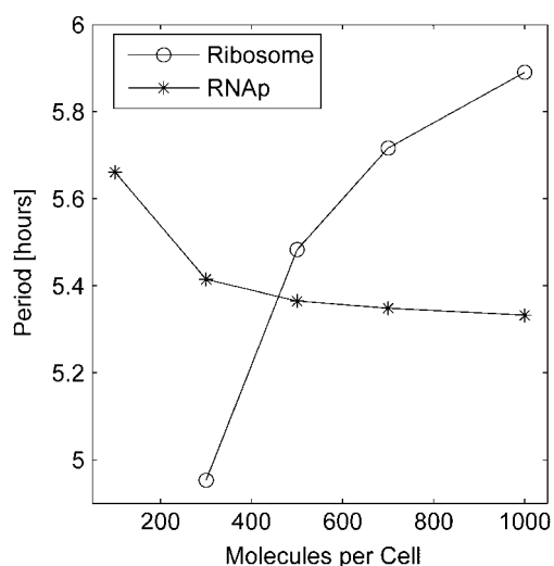
FIGURE 8 Effect of initial ribosome and RNA polymerase numbers on the period of oscillation. The number of initial RNA polymerases and ribosomes is, respectively, varied from 100 to 1000 and 300 to 1000 molecules.
